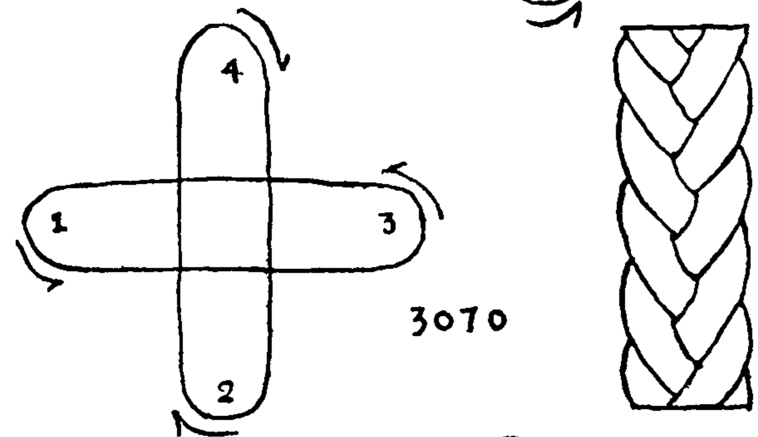
#3069 (6-STRAND ROUND) (All strands move to right.)
